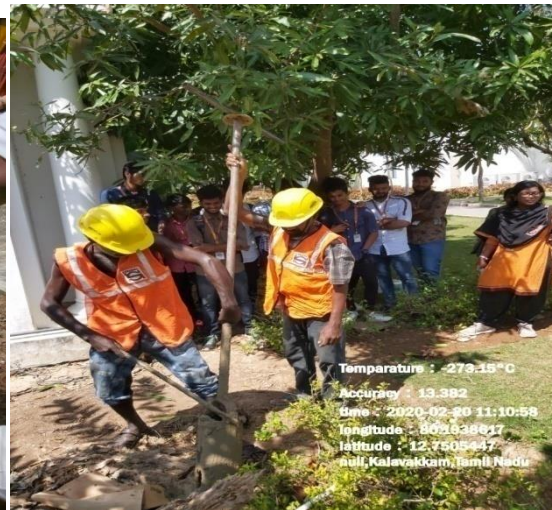
Field Visit – Lime Grouting for Soil Stabilisation – 20.02.2020
