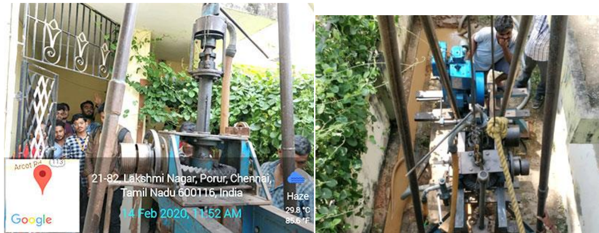
Geotechnical Investigation Camp 2020 – Porur, Chennai
